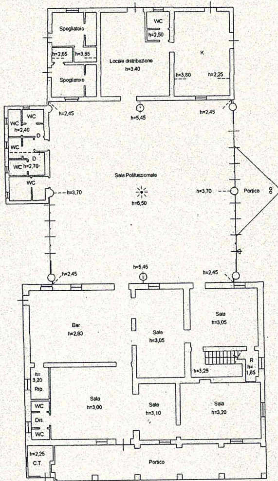
PIANO TERRA
