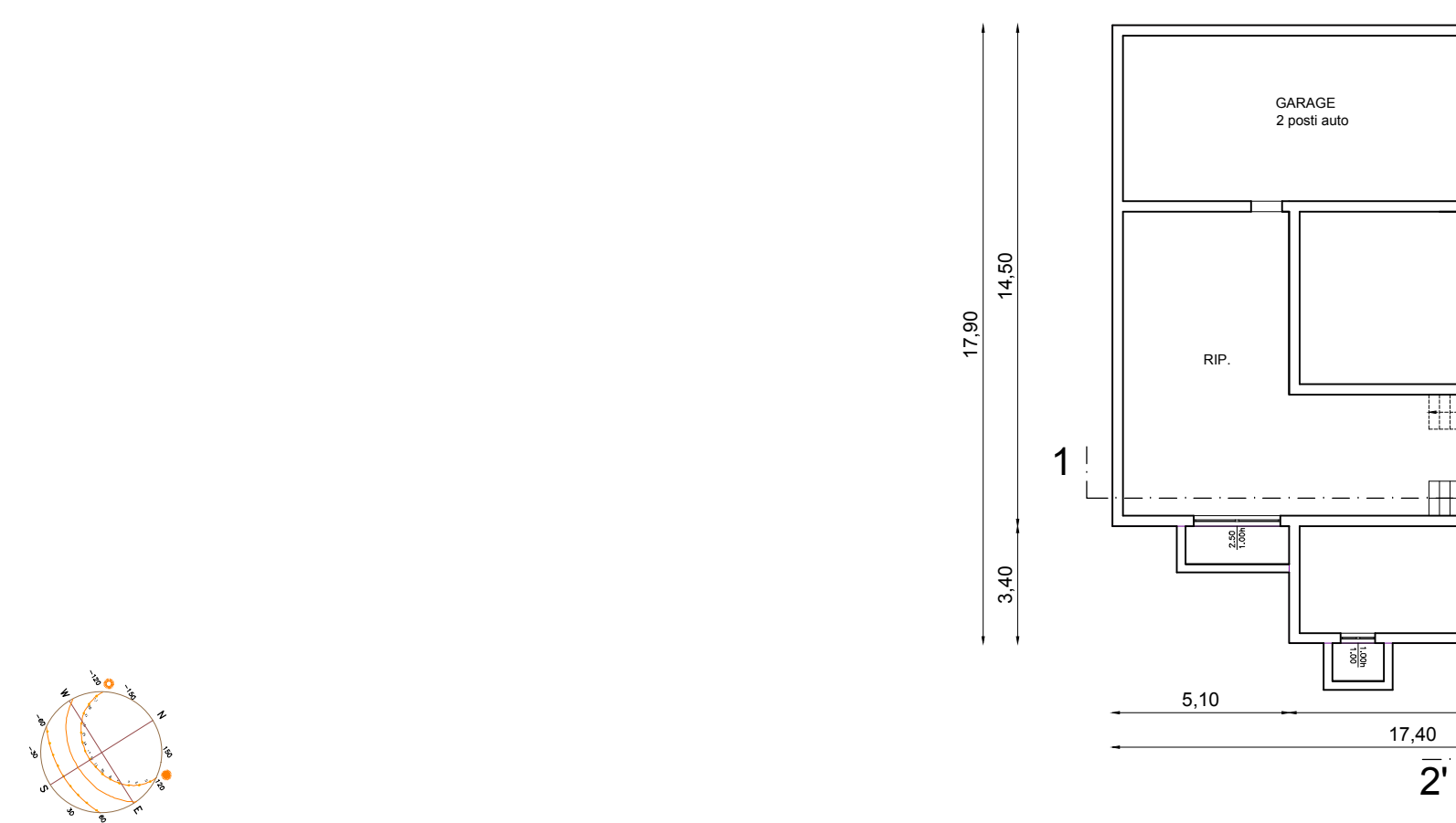
PIANO INTERRATO
