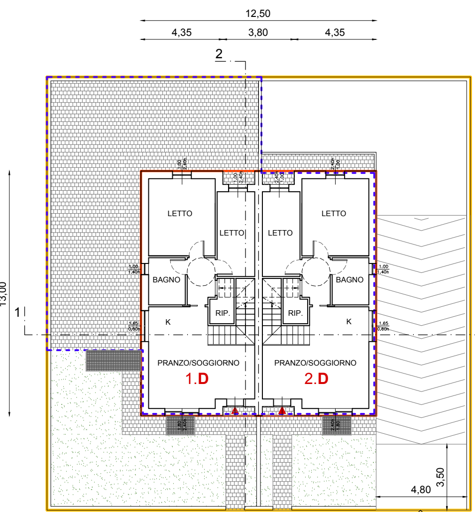
PIANO TERRA
