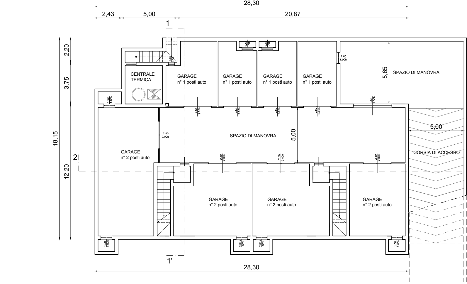
PIANO INTERRATO
