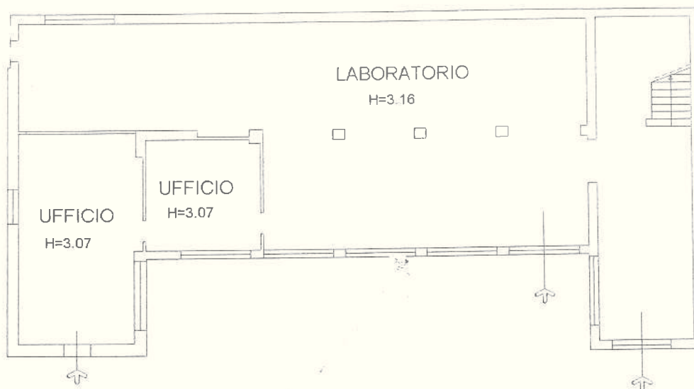
PIANO TERRA
